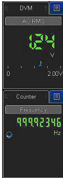
Figure 25. DVM and counter takes advantage of separate signal paths to provide measurements without a trigger, while still using the scope probes.
